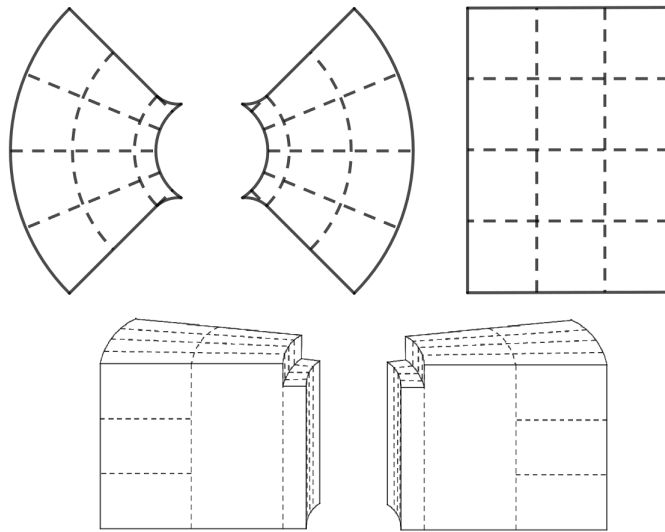
Figure 4: Advanced model geometry used to describe the rotor. Top left is a front view, top right is a side view (external sub-sectors) and bottom is a tilted view of the sectors. Only the 4 external part sectors are divided in 3 sub-sectors each. The chamfers are visible on the inner radius.
