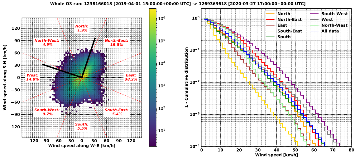
Figure 19: Wind statistics as measured by the EGO weather station during the O3 run. The left plot shows the joint distribution of the wind speed and orientation, with the two black bars showing the directions of the two arms of the Virgo detector. The right plot shows the complementary cumulative distribution of the wind speed for each of the eight quadrants of the wind rose.
