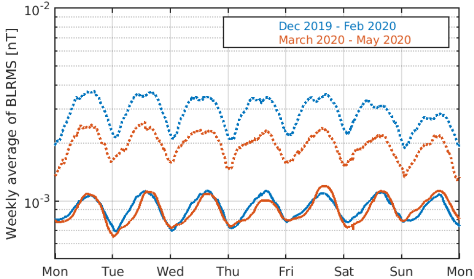
Figure 24: Weekly averaged magnetic field band-limited RMS value computed in two frequency bands: 1 to 6 Hz (dashed) and 18 to 24 Hz (solid). Magnetic field intensity is measured externally of Virgo experimental buildings, in the reference period between December 2019 and February 2020 (blue curves) and in the period between March 15 and May 15 (red curves) which corresponds to reduced anthropogenic activity within and outside of EGO because of the COVID-19 pandemics.
