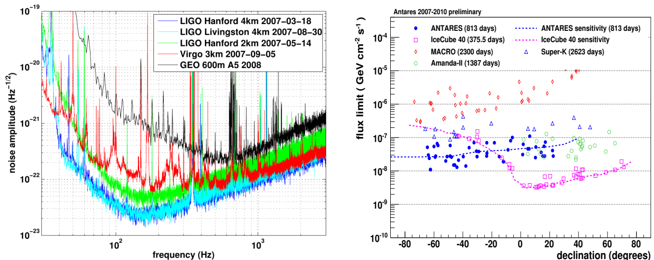
FIG. 3 Left: Best detector noise spectra from the LIGO and Virgo associated with the S5/VSR1 data set (2007) along with that of GEO (2008). This figure is taken from (Abadie et al. , 2011). Right: Current experimental sensitivities to differential cosmic neutrino flux E^{-2} \frac{dN}{dE} (solid lines) and limits (points) in function of declination for time-integrated searches of point-like sources. The figure shows the results of AMANDA-II (Abbasi et al. , 2009) and its successor IceCube, in its 22-string (Abbasi et al. (2009); Abbasi et al. (2009)) and 40-string (Abbasi et al. , 2011) configurations, as well as those of ANTARES; also displayed are the limits from the MACRO (Ambrosio et al. , 2001) and Super-Kamiokande (Thrane et al. , 2009) experiments, which are not principally devoted to neutrino astronomy. Figure taken from (Dornic, 2011).
