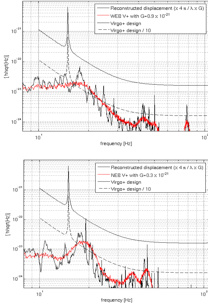
Figure 5.3 Top: Estimation of diffused light noise from WE for Virgo+MS (red) compared to the V+MS design (black) and the design divided by 10 (dashed). The coupling factor has been rescaled with respect to Virgo to account for the new ITF parameters: F=150 and T_{end}=3ppm . Bottom: same for NE.
