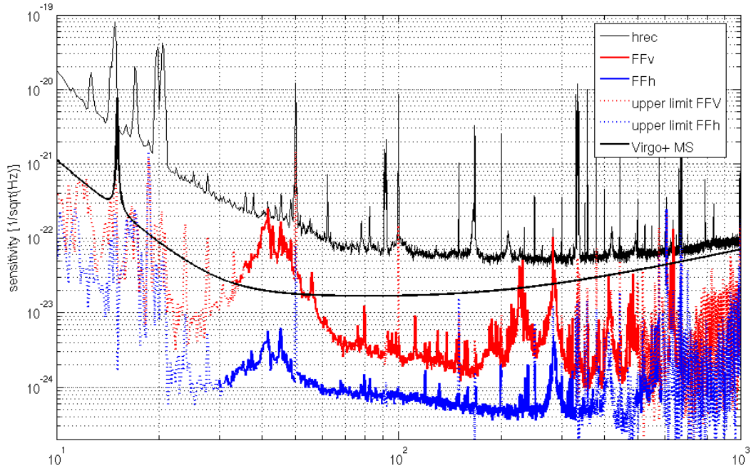
Figure 8.1: Contribution of jitter noise of the input beam measured along the vertical direction (red) and horizontal direction (blue) compared to V+MS design. The noise around 40Hz is associated to the vertical resonance of the EIB; structures between 200 and 500Hz are associated to mechanical mounts of the optics of BMS; between 70Hz and 200Hz the measurement is likely limited by the noise of the BMS quadrants. The horizontal jitter noise is smaller or less coupled to the sensitivity. This has not been yet understood.
