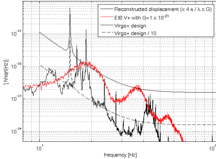
Figure 5.5 : Estimate of diffused light noise from EIB for Virgo+MS (red) compared to the design (black) and the design divided by ten (dashed). The projected noise (red) is an upper Limit based on the measured coupling factor upper limit ( G \leq 1 \times 10^{-21} ).
