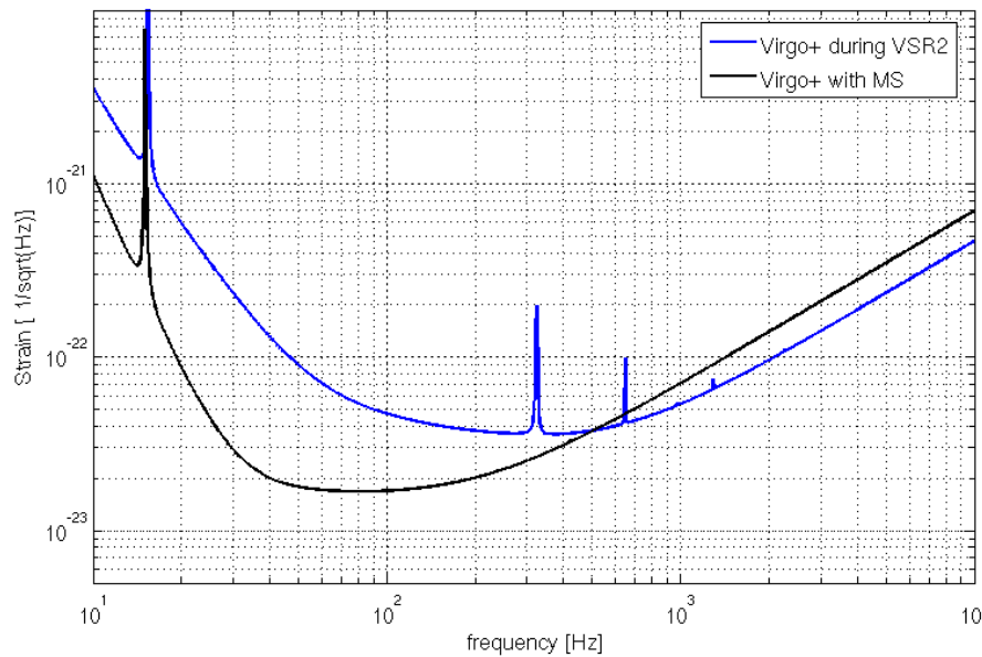
Figure 1.2: Virgo+ (blue) and Virgo+MS (black) design curves. The sight range computed for NS-NS of 1.4 solar masses with these curves is 13Mpc for Virgo+ and 47Mpc for Virgo+MS. This plot is taken from reference [3].
