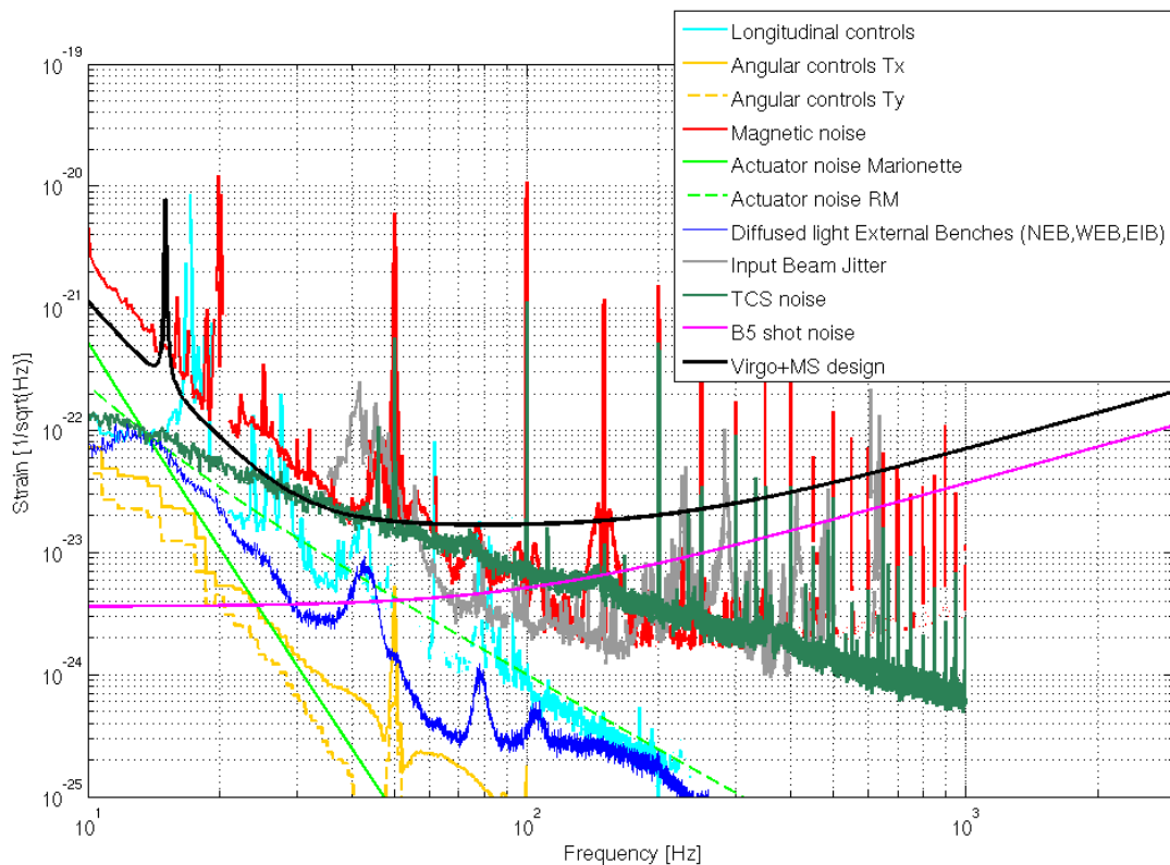
Figure 11.1: superposition of expected noise contributions to V+MS described in previous chapters.
