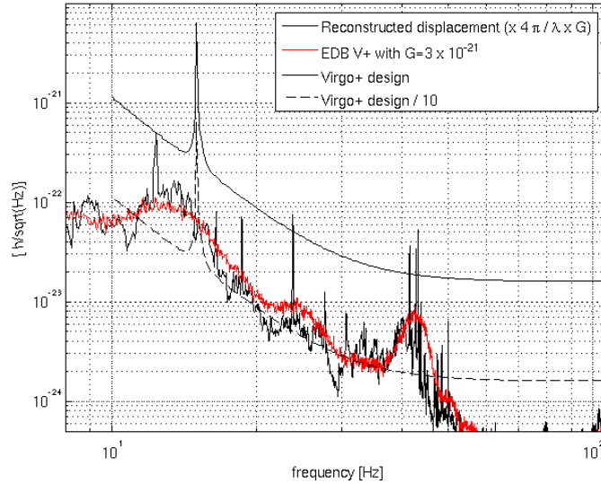
Figure 5.4 : Estimation of diffused light noise from EDB for Virgo+MS (red) compared to the design (black) and the design divided by ten (dashed). This noise is dominated by B5 and B1p photodiode contribution. The coupling factor of B5 has been rescaled with respect to Virgo measurement to take into account the new finesse ( F=150 ). It is assumed that some improvements are done on B1s path leading to a reduction of its diffused light noise by at least a factor 10 (see text). B1s noise is therefore expected to be a factor 3 below B5 noise. B1p coupling is expected to remain the same and it could be identical to B5 noise. Thus, shown projected noise is expected to be dominated by diffused light from B1p and B5 beams in similar amount.
