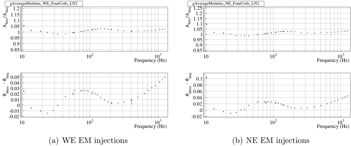
Figure 8: Comparison of the reconstructed raw h(t) vs the h(t) injected with the WE and NE electromagnetic actuators. This is the average of weekly measurements.
