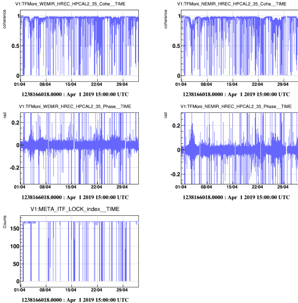
Figure 5: Monitoring of the sign of h(t) with the photon calibration permanent lines during a month (April 2019).. The last line shows the time series of ITF lock index for reference. The first lines show the Time series of the coherence (top) and phase (middle) of the transfer functions at the frequency of the permanent line from the injected PCal h(t) signal to the reconstructed raw h(t) signal (left for WE and right for NE).
