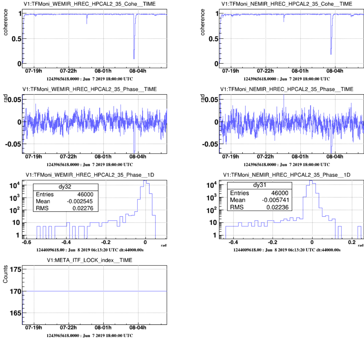
Figure 6: Monitoring of the sign of h(t) with the photon calibrators during a lock segment on June 7th 2019. The last line shows the ITF lock index for reference. First and second lines show the time series of the coherence (first line) and phase (second lines) of the transfer functions from the injected PCal h(t) signal to the reconstructed raw h(t) signal (left for WE and right for NE). The third line shows the distribution of the phase (zoomed without a few outliers at the time of low coherence).
