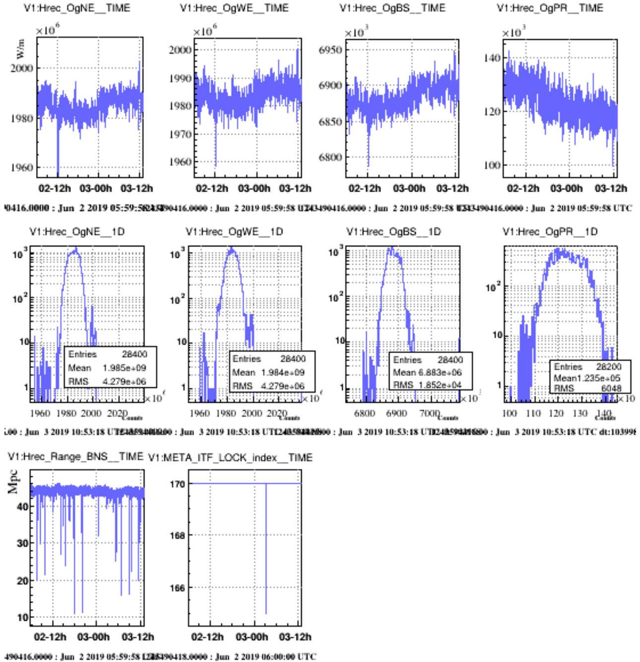
Figure 2: Typical fluctuations of the optical gains for NE, WE, BS and PR. First line: time series of optical gains of NE, WE, BS and PR. Second line: distributions of the NE, WE, BS and PR optical gains. Third line: computed range and lock state in the same time window.
