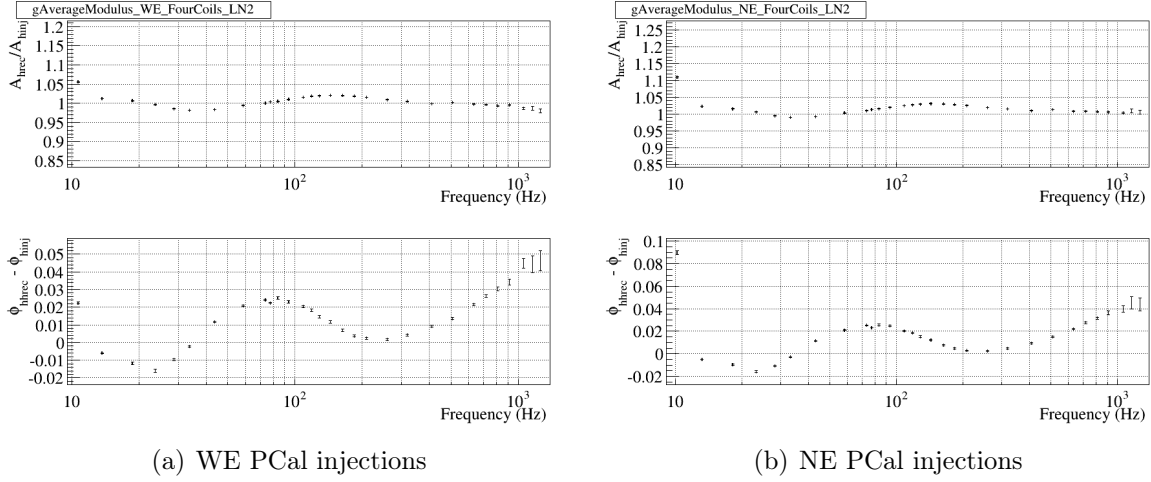
Figure 7: Comparison of the reconstructed raw h(t) vs the h(t) injected with the WE and NE PCals. This is the average of weekly measurements.
