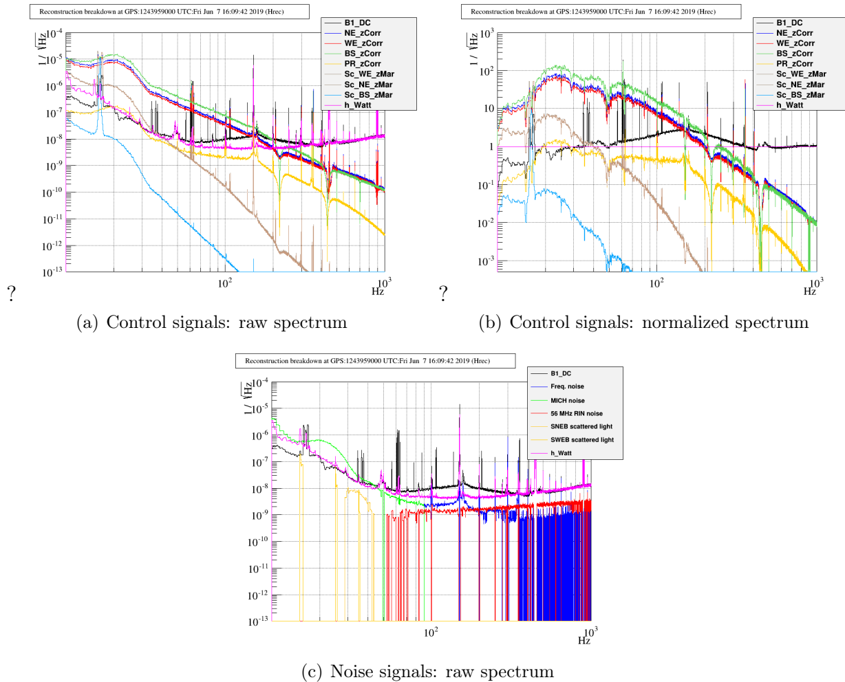
Figure 1: typical spectrum of the signals involved in the reconstruction (GPS 1243959000, on June 7th 2019). Top: control signals raw spectrum (left) and normalized to the h(t) spectrum (right) to see their relative contributions. Bottom: noise witness signals raw spectrum.
