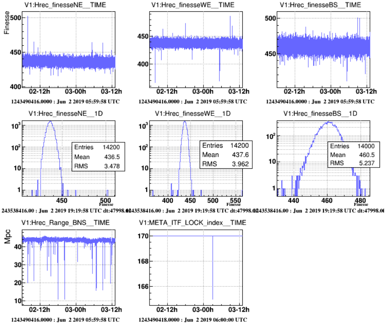
Figure 3: Typical fluctuations of the fitnesses for NE, WE, BS. First line: time series of fitnesses NE, WE, BS. Second line: distributions of the NE, WE, BS fitnesses. Third line: computed range and lock state in the same time window.
