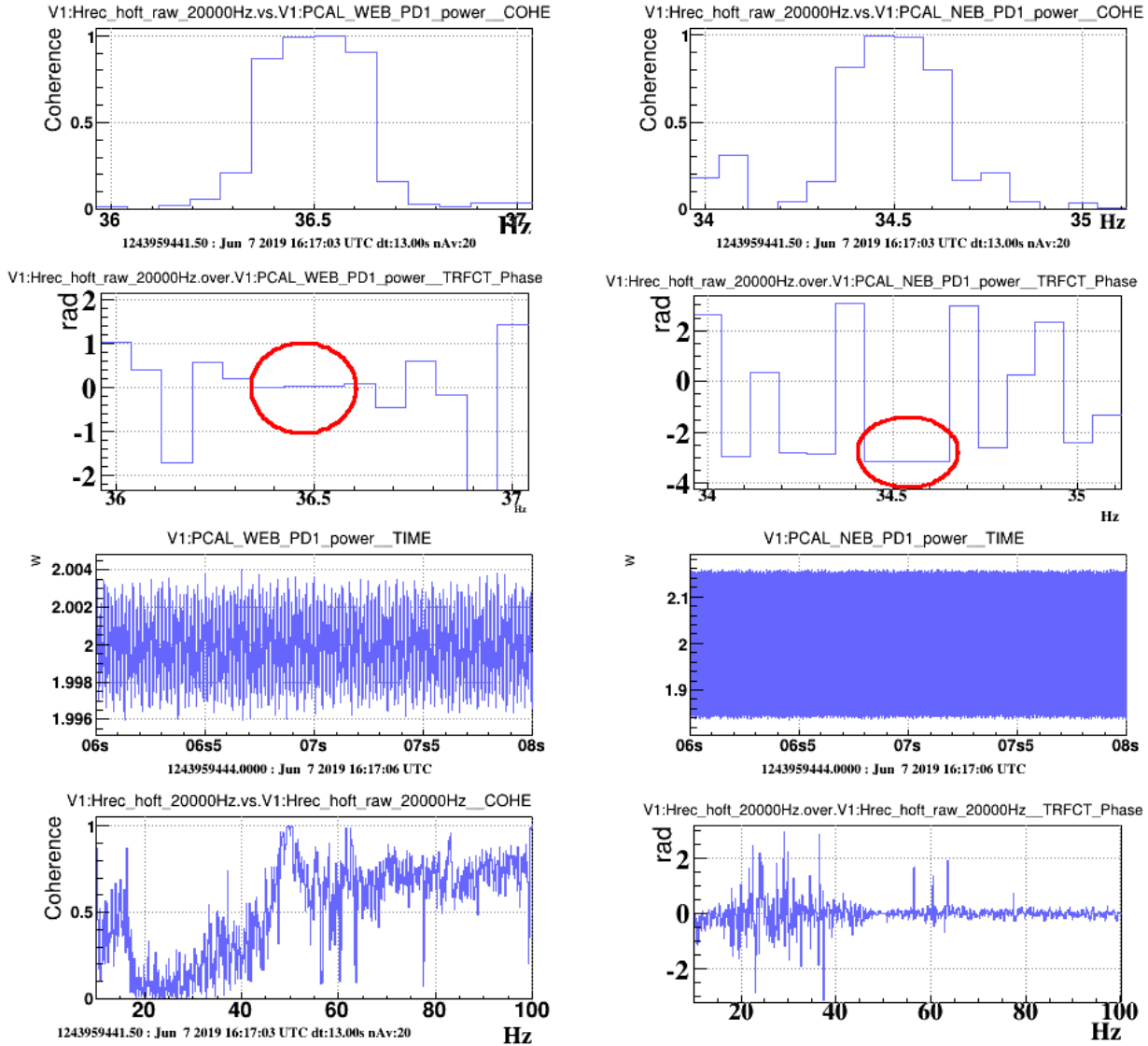
Figure 4: Validation of the sign of h(t) . The first two lines show the coherence and phase of the transfer function from the PCal power to the h(t) channel including hardware injections (i.e. from PCAL_WEB_PD1_power to Hrec_hoft_raw_20000Hz). Left for WE and right for NE PCal. The phase points with good coherence at the PCal calibration line frequency are highlighted. The third line shows the time series of the PCal sensing channels, which give positive values. The last line shows the coherence and phase of the transfer function from Hrec_hoft_raw_20000Hz to Hrec_hoft_20000Hz: they are indeed in phase.,
