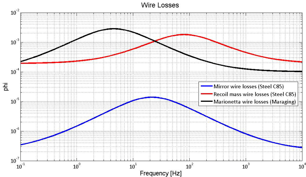
Figure 5: Overall loss factors of the wires in the Monolithic last stage suspension
