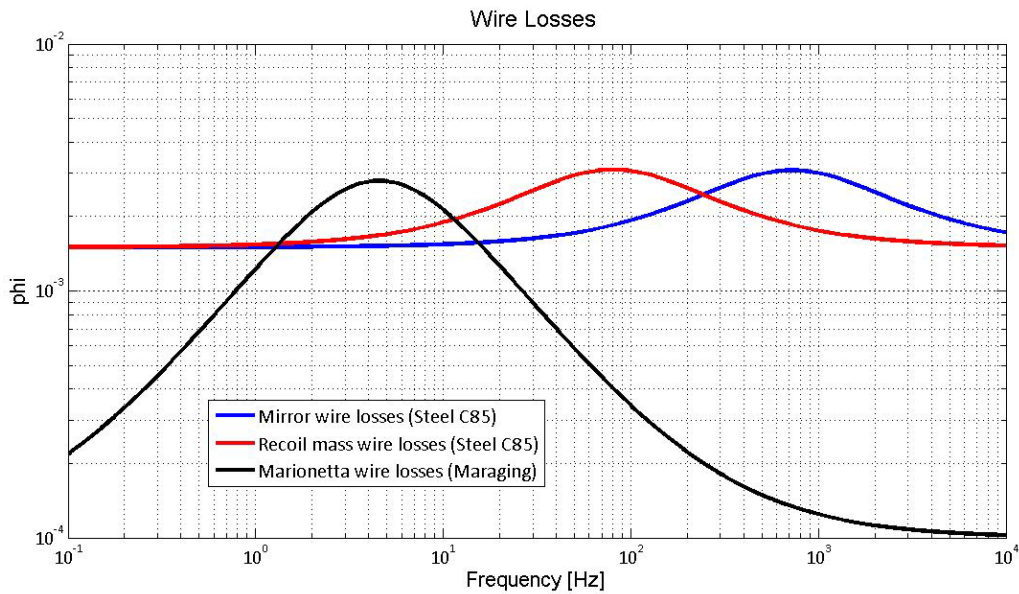
Figure 6: Overall loss factor of the suspension wires the Virgo+ without MS
