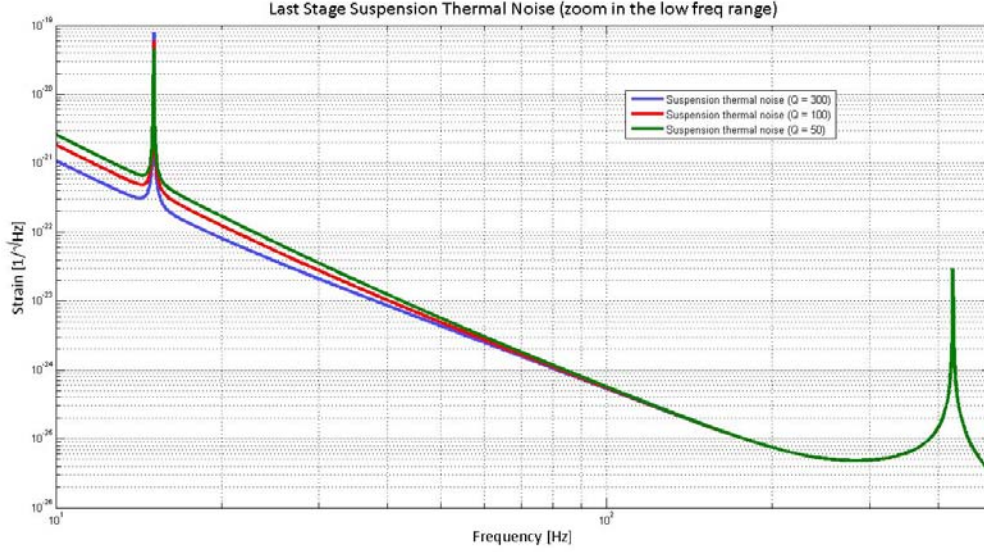
Figure 7: Monolithic Last Stage Suspensions Thermal noise with 3 possible viscous dissipations on the marionette.
