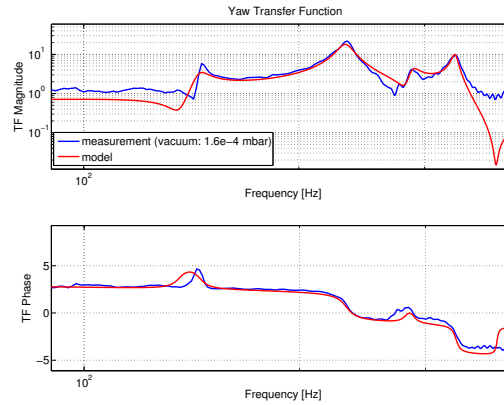
Figure 47: Parabolic mirror M2 mount: comparison between measured transfer function and theoretical model in yaw (vacuum condition).
