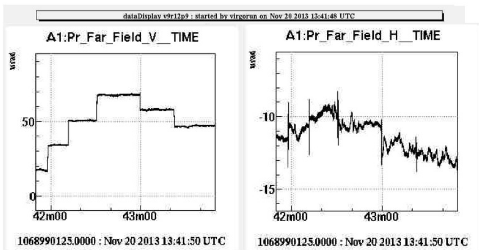
Figure 22: Motion in pitch of the M2 mount: (left) pitch signal and (right) yaw signal.
