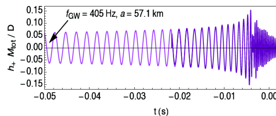
FIGURE 4. Example of the expected GW waveform from the coalescence of a black-hole binary as predicted by the post-Newtonian theory. Credits: [18]
