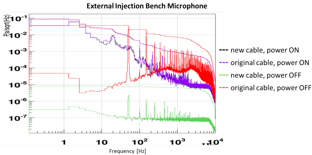
Figure 1: Amplitude Spectra and rms with new and old connecting cables. Each pair of curves shows the amplitude spectrum and cumulative rms (rms is displayed as the square root of cumulative integral of the power spectrum, integrated from high to low frequencies) of a particular configuration (see legend).
