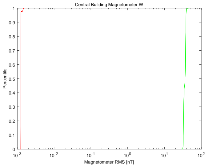
Figure 3: Cumulative distributions of rms for an example magnetometer. The green curve shows the distribution of rms over a one week period when the magnetometer was on. The red curve shows the distribution of rms for a day that it was off. Note that the distributions are separated by four orders of magnitude.
