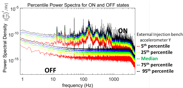
Figure 6: Percentile Power Spectra for an Example Accelerometer. Each set of percentile spectra is calculated from the power spectra of 100 successive 5-second intervals. The lower set of spectra is from a time when the sensor was off and the upper set of spectra is from a time when the sensor was on.
