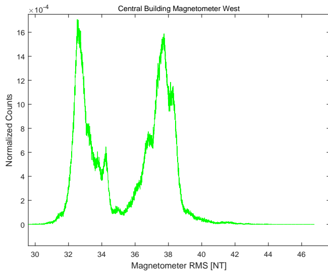
Figure 4: Binned, normalized distribution of Power-ON RMS for Central Building Magnetometer West. This distribution was computed for a week of rms trend data.
