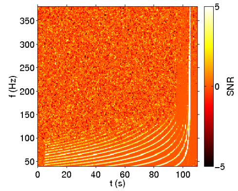
(b) EBBH A waveform
