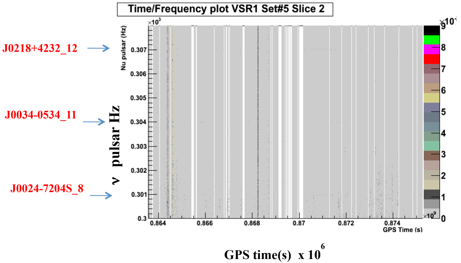
Fig.4 Time/Frequency plot of these data between 300 and 308Hz
