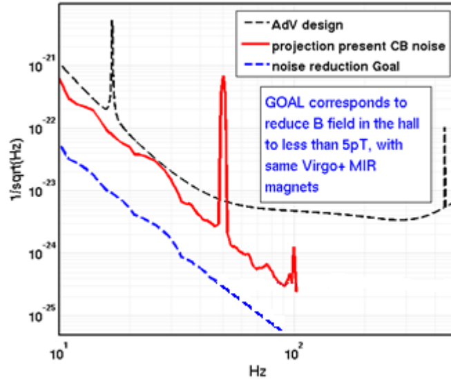
Figure 2. Advanced Virgo Strain noise. Fundamental noises (black dashed line) are compared with the noise contribution of the environmental magnetic field: (RED continuous line) projection of Central Building magnetic noise; (blue dashed) projection assuming a magnetic noise of 5pT.
