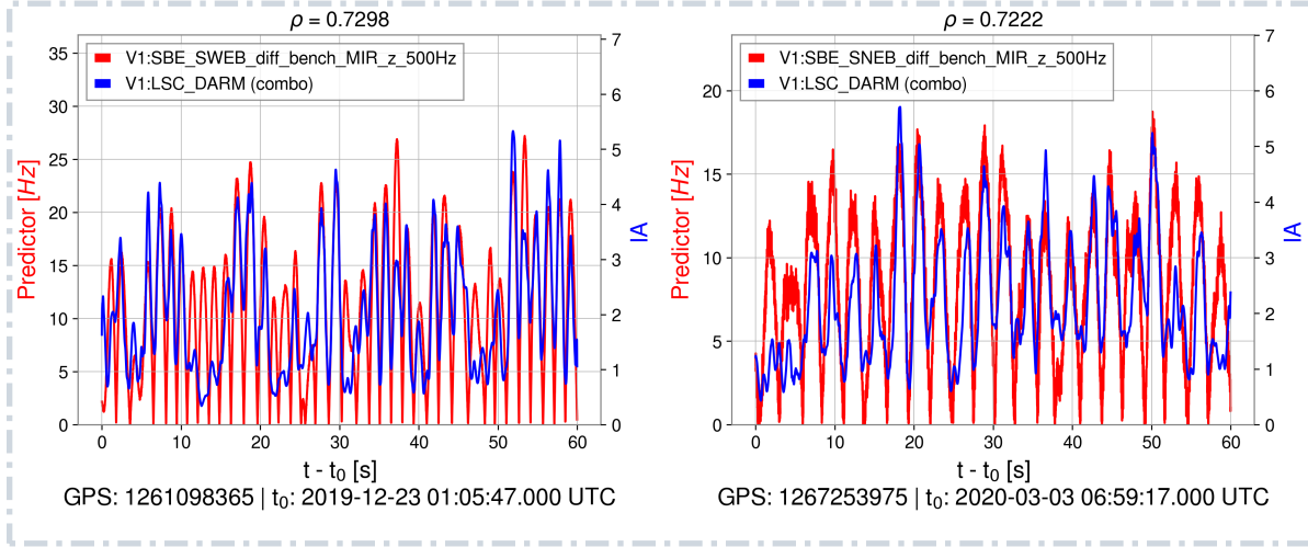
Figure 19: In red is the culprit’s predictor, i.e. Equation 3 for the relative motion (diff) between the suspended end bench and the end mirror (BENCH-MIRROR) of the West end (left) and North end (right). The sum of the IA of the first two modes of DARM, extracted by tvf-EMD is shown in blue.
