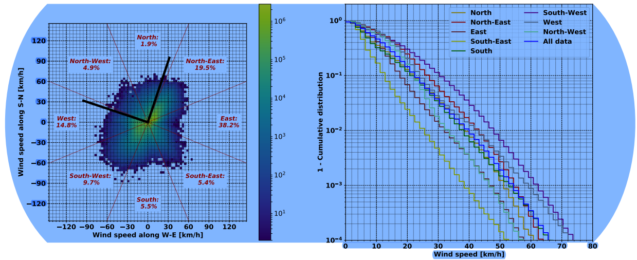
Figure 20: Wind statistics as measured by the EGO weather station during the O3 run. The left plot shows the joint distribution of the wind speed and orientation, with the two black bars showing the directions of the two arms of the Virgo detector. The right plot shows the complementary cumulative distribution of the wind speed for each of the eight quadrants of the wind rose.
