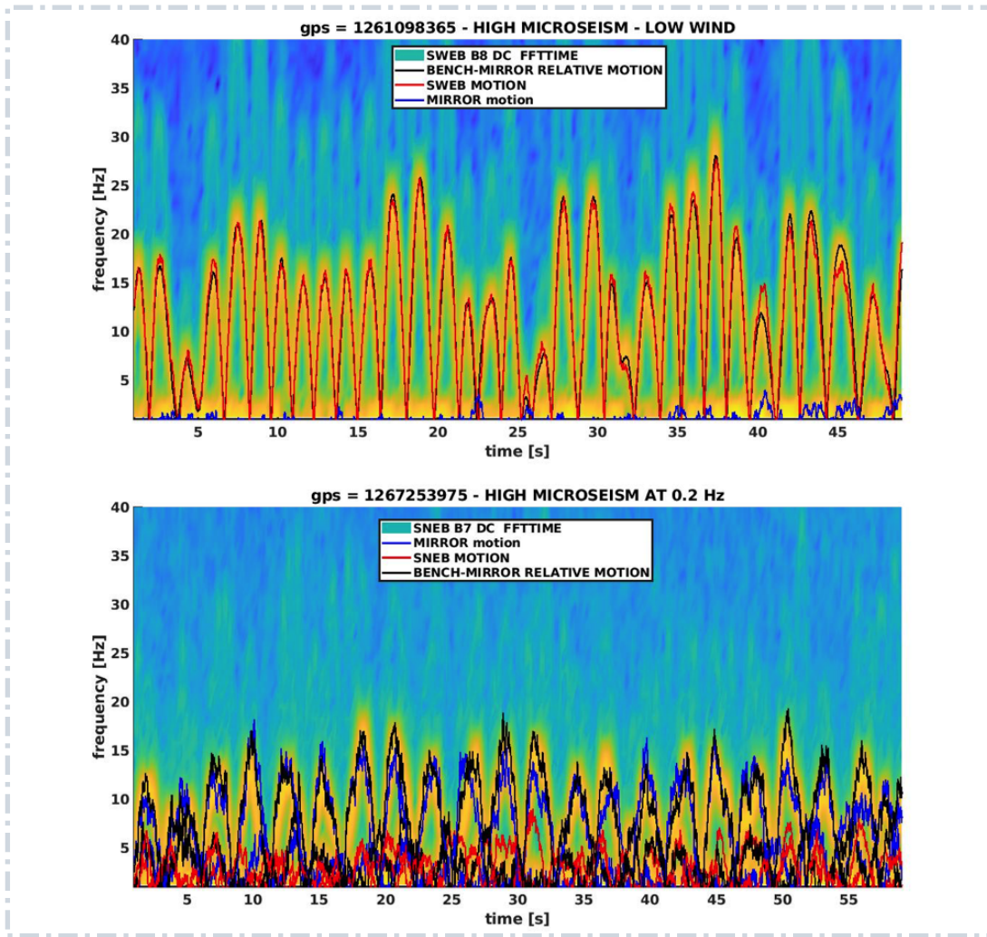
Figure 18: Spectrograms of the light transmitted at the end of the arm cavities and detected by photodiodes located behind, on suspended benches – top plot: west arm, B8 photodiode, SWEB bench; bottom plot: north arm, B7 photodiode, SNEB bench. The typical pattern of scattered light noise (arches) – both first order and second order (higher frequencies) – is visible. On the SWEB plot, arch spacing and amplitude correspond to half the period of marine microseism at Virgo ( \sim 3 s) and a ground velocity of about 8 \mu\text{m/s} . The predictor for BENCH-MIRROR is shown in black, while the predictors computed from mirror and bench motions are shown in blue and red, respectively. The overlap shows that BENCH-MIRROR is the best predictor of scattered light, closely matching the observed arches.
