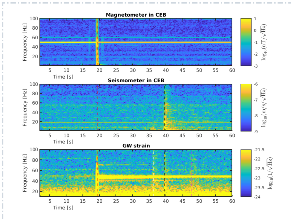
Figure 26: Impact on the Virgo environment and detector of one lightning strike which occurred 6 to 10 km away from Virgo buildings on November 15, 2019 at 23:25:51 UTC. The spectrograms of a few relevant signals are shown. (Top) A prompt magnetic transient is detected by magnetometers at the time of the event, marked by the red vertical line. (Middle) A few seconds later, a seismic (and acoustic, not shown) transient is detected in the central experimental area, marked by the black vertical line. The bottom spectrogram shows the reconstructed GW strain during the same time interval. The red vertical line marks the lightning strike occurrence, the black, magenta and white vertical lines mark the occurrence of seismic transients detected in the CEB, NEB and WEB, respectively.
