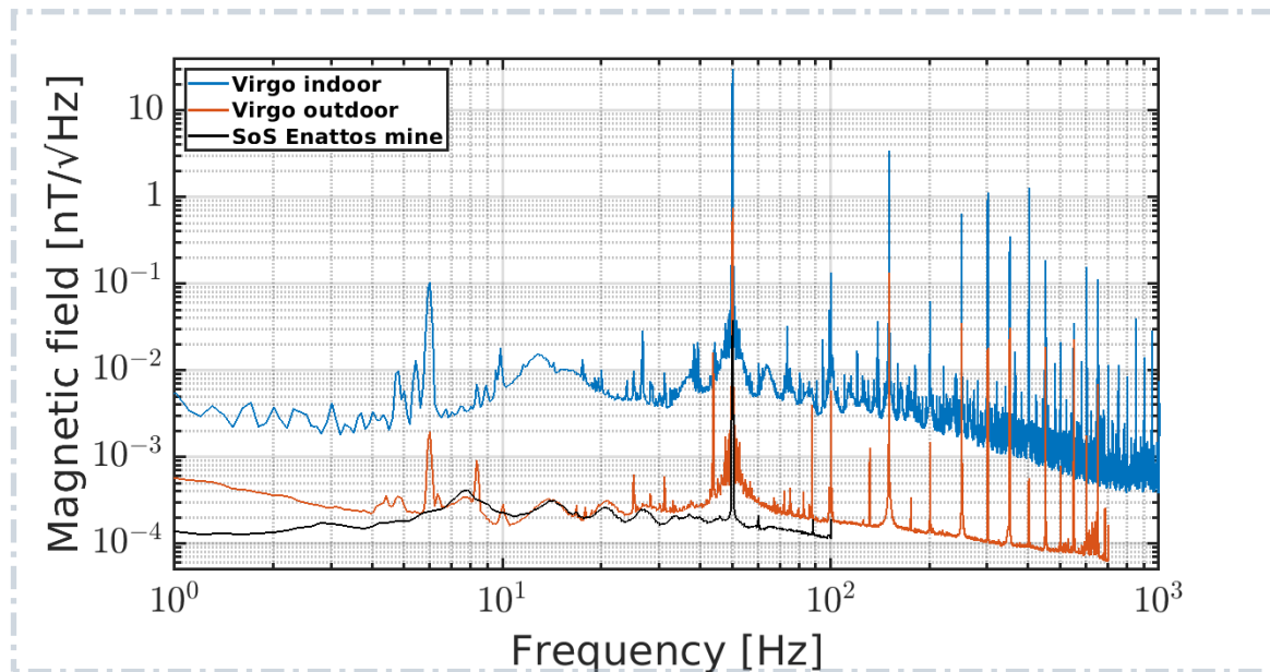
Figure 24: Amplitude spectral densities of indoor (blue curve) and outdoor (red curve) magnetometers at EGO and at Sos Enattos mine in Sardinia (black curve). The quiet Sos Enattos location shows evidence of Schumann resonances peaked at approximately 8, 14, 21, 27 and 33 Hz.
