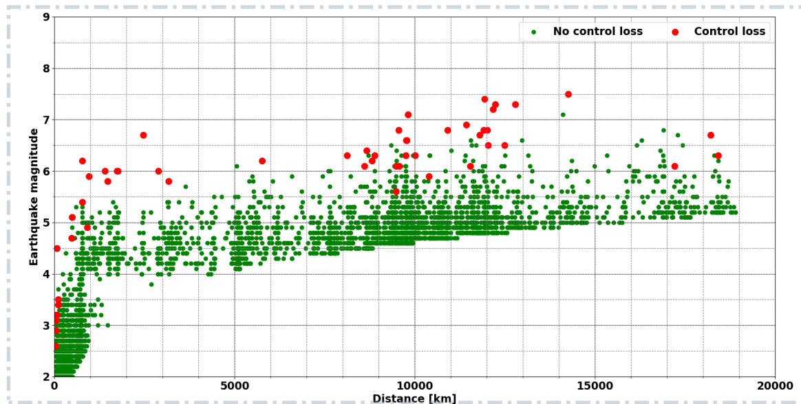
Figure 12: Distribution of earthquakes in the plane distance-magnitude during the O3 run. The earthquakes that caused a control loss (did not cause a control loss) are represented with red (green) dots. The lack of points below the main bulk of earthquakes is due to the ranking cut, set at 0.02.
