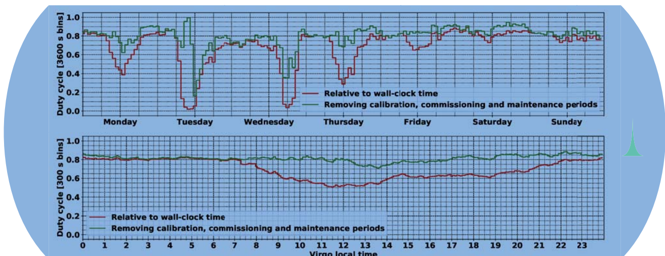
Figure 10: Average weekly (top) and daily (bottom) duty cycle of the Virgo detector during the O3 run. The red curve uses the elapsed real time as normalization, while the green one is produced excluding the times spent doing calibration, commissioning or maintenance, three activities that are incompatible with Science-mode data taking.
