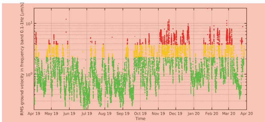
Figure 4: Evolution during O3 of seismic RMS in the 0.1 to 1 Hz frequency band. Data colored in yellow and red exceed the 75 th and 90 th percentile, respectively.
