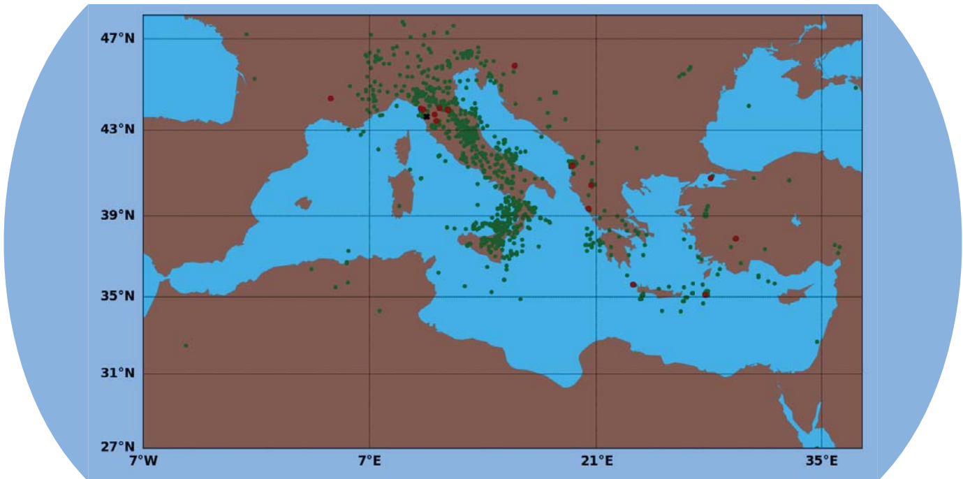
Figure 14: Zoom on the Mediterranean area of the map shown in Fig. 13 above. It shows the earthquakes nearby Virgo (whose site, EGO, is marked by a black cross) recorded during the O3 run. The earthquakes that caused a control loss (did not cause a control loss) are represented with red (green) dots.
