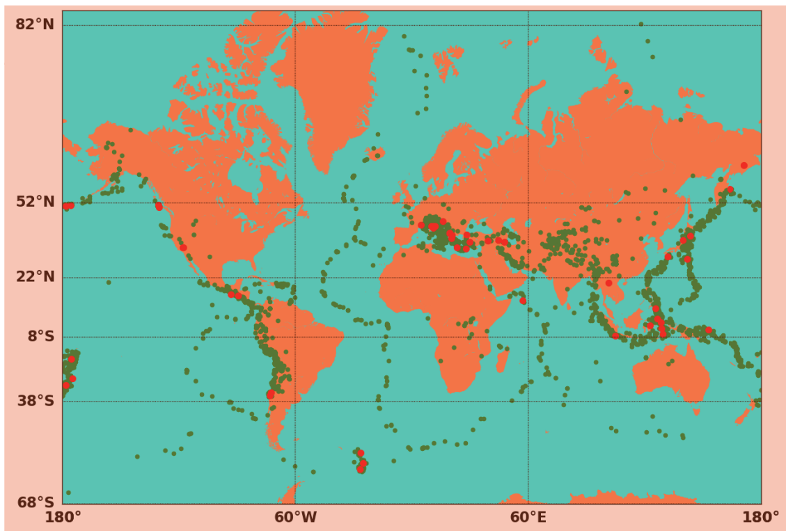
Figure 13: Location of the O3 earthquakes used in this study (ranking greater than 0.02). The earthquakes that caused a control loss (did not cause a control loss) are represented with red (green) dots.
