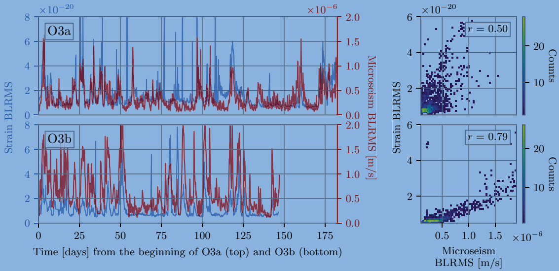
Figure 16: Correlation between the low frequency noise in Virgo GW strain and the microseism induced by the sea activity; top row for for O3a and bottom for O3b. Left: in blue the time series of the strain BLRMS in band [10, 20] Hz and in red that of the BLRMS in band [0.1, 1] Hz of a CEB seismometer, mostly influenced by the sea activity. Right: 2D-histograms of the correlation between the two BLRMS, where the colorscale counts, for every pixel in this map, how many data points have the corresponding values of strain and microseism BLRMS. The annotations in the top-right corners report the values of their Pearson correlation coefficient r .
