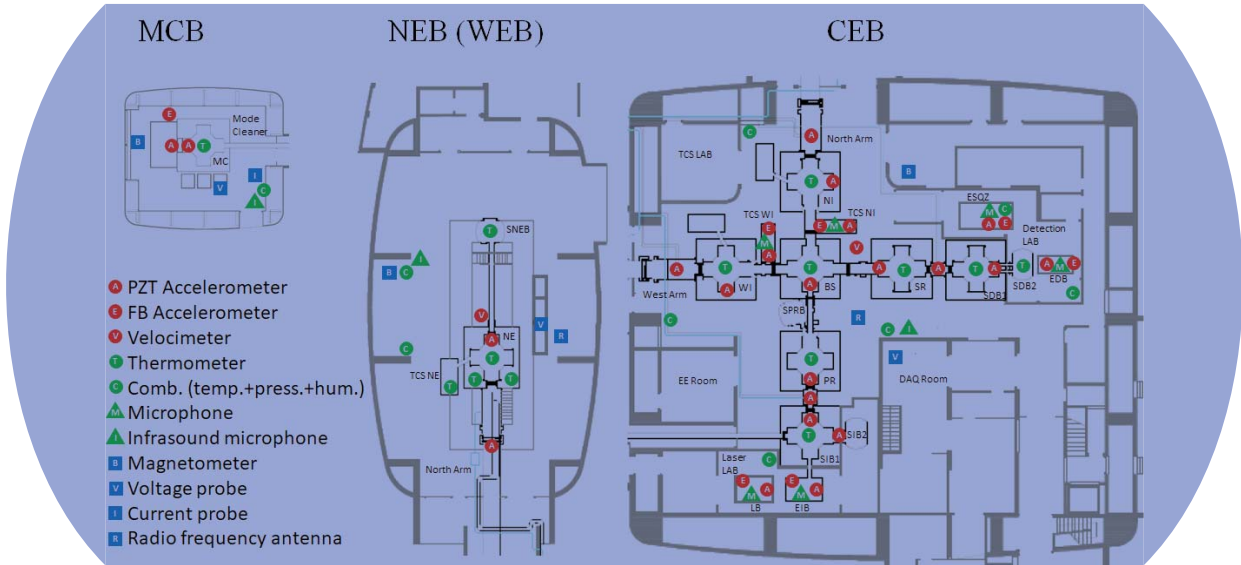
Figure 1: Location of the probes used for the Virgo environmental monitoring system. Maps of most relevant building are shown: left MCB, middle NEB, right CEB. The WEB is very similar to NEB and is not shown.
