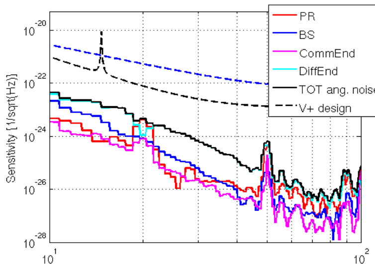
Figure 3.8: simulated control noise for the ty direction
