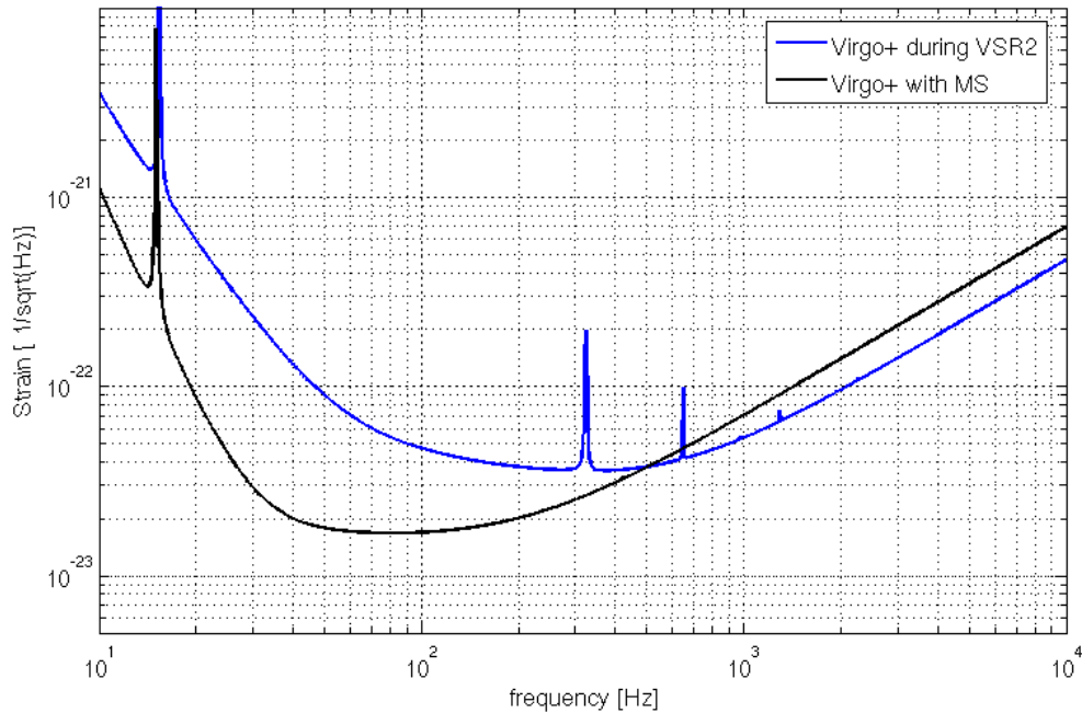
Figure 1.2: Virgo+ (blue) and Virgo+MS (black) design curves. The sigh range computed for NS-NS of 1.4 solar masses with these curves is 13Mpc for Virgo+ and 47Mpc for Virgo+MS. This plot is taken from reference [3].
