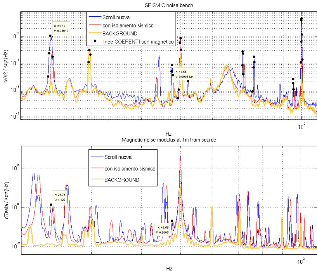
Figure 5: Scroll pump, test of magnetic versus seismic noise emissions and their measurement.
