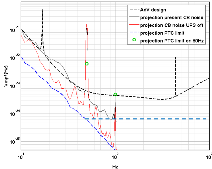
Figure 2. Taken from VIR-0135B-11 . The dashed blue line depicts the hrec noise associated to a magnetic field at the AdV test masses which equals the limit values listed in Table 1.
