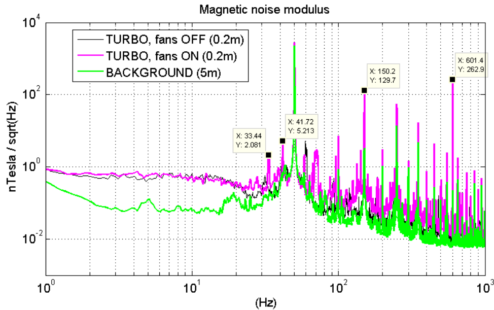
Figure 16. Magnetic noise from the cooling fans of the Turbo pump. Measurement at 0.2m distance.
