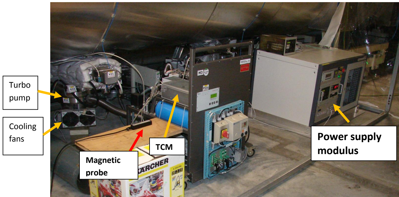
Figure 3. Setup at 1200N. Vacuum pumping station at 1200N along the Virgo N tube. The magnetic noise background is about 10 times larger than in the 1500N Lab. We measured the background noise approximately in the photographer position (i.e. about 5m from TMC and 7m from the power supply modulus, and 60cm from ground).
