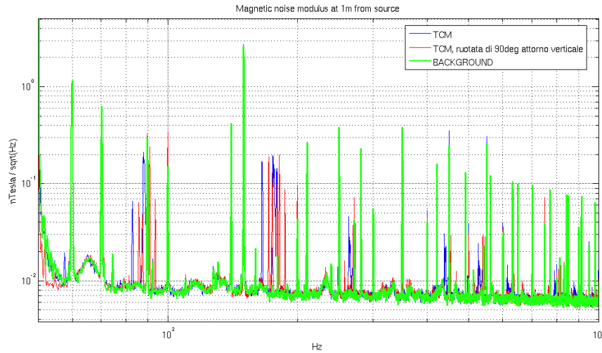
Figure 13. Magnetic noise at 1m from one TCM running standalone (switched on, but not connected to its turbo pump).
