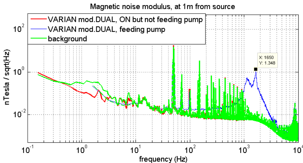
Figura 12. VARIAN-DUAL connected to ion pump.
