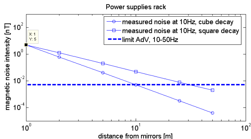
Figure 17. Evaluation of safe distance from suspended mirrors of each vacuum rack device based on measured noise extrapolated with cubic (circles) and square (squares) laws and the set limits (dashed lines).
