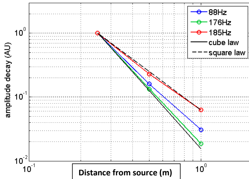
Figure 7. Rough measurement of the decay of the B field intensity with increasing distance from the source (one TMC modulus). The measurement is done for three different frequencies.
