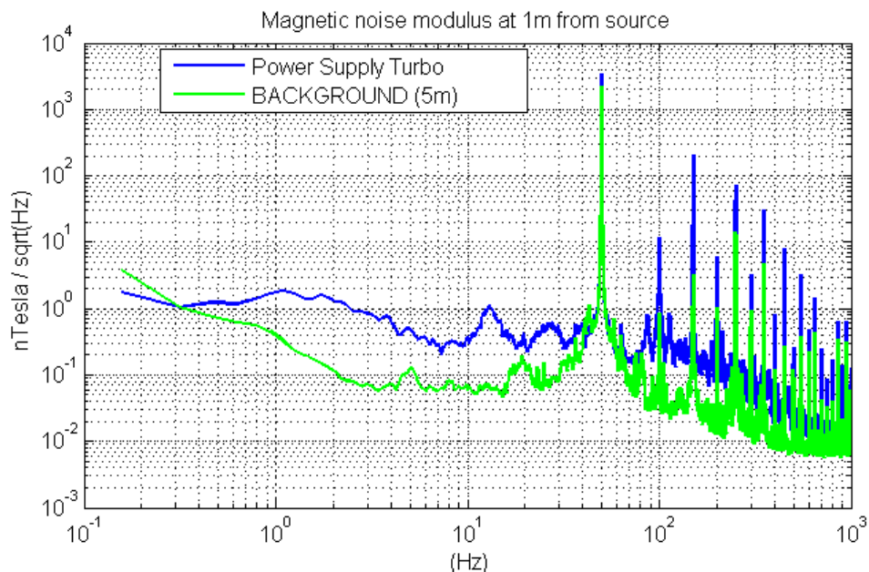
Figure 16. Power supply modulus.
