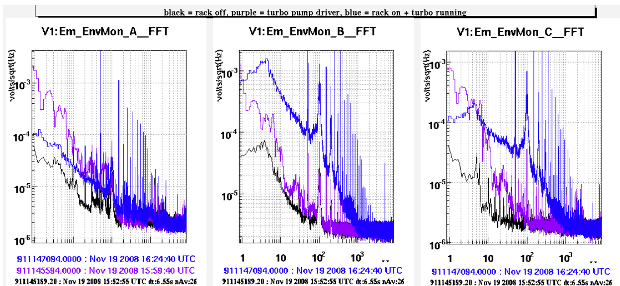
Figure 1: plot from eLog 21327 . Measurement of magnetic field at 1m from SR rack: black= all rack OFF, blue=RACK ON, purple = only TCM on (powered separately on UPS). Vertical axis calibration: 1\text{E-}4 V corresponds to 1\text{nT} .
