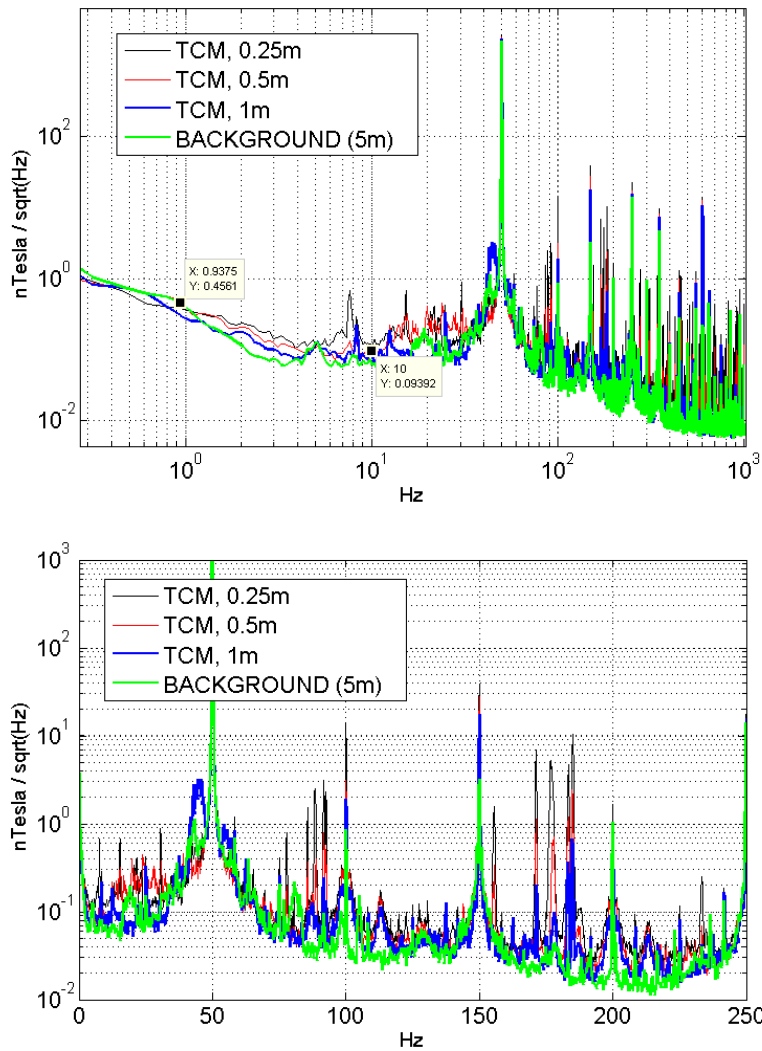
Figure 14. Magnetic noise of one TCM connected to its turbo pump.
