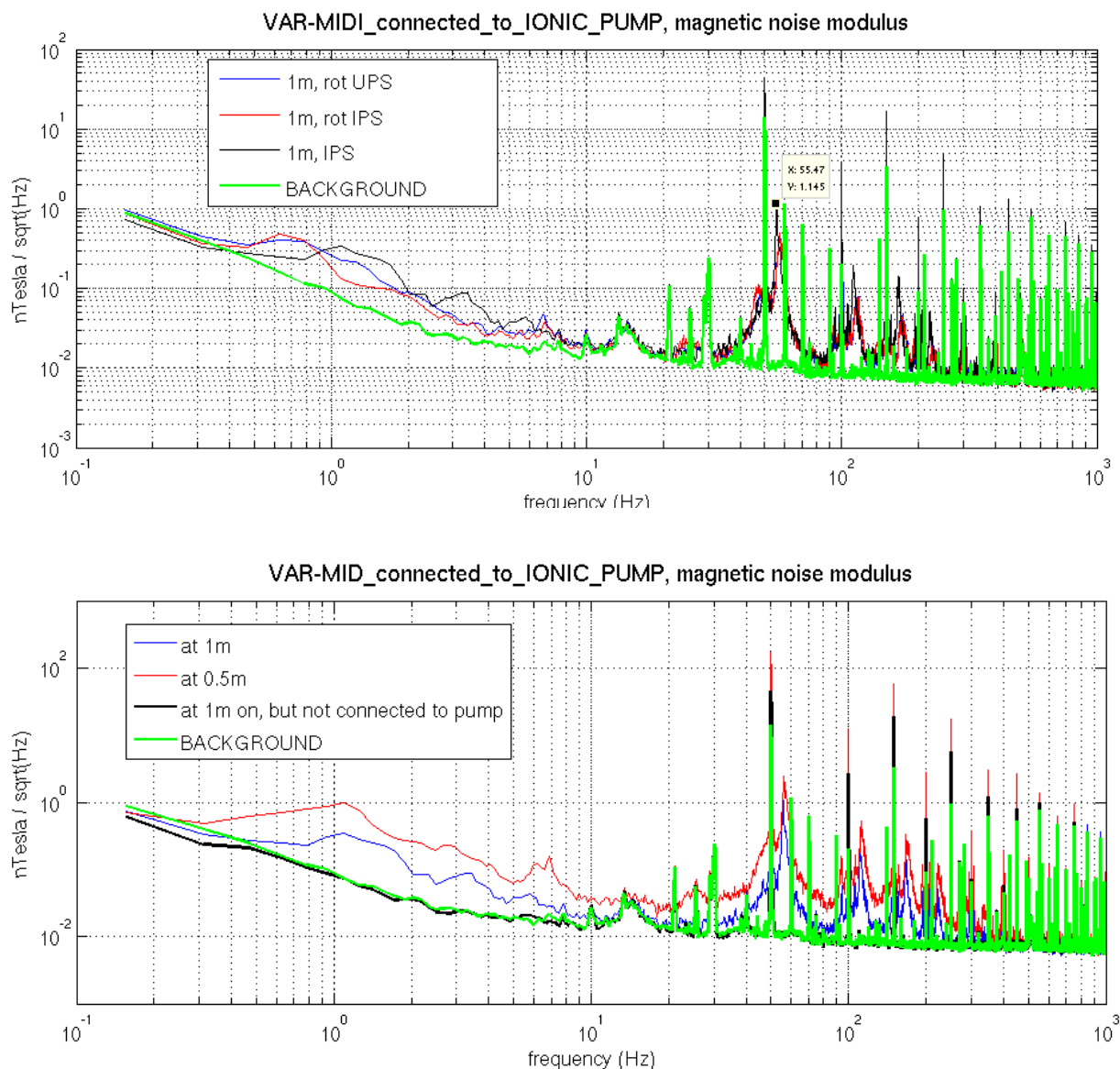
Figure 11. VARIAN-MIDI connected to ion pump. TOP: magnetic noise at 1m distance, BOTTOM: magnetic noise at two different distances.
