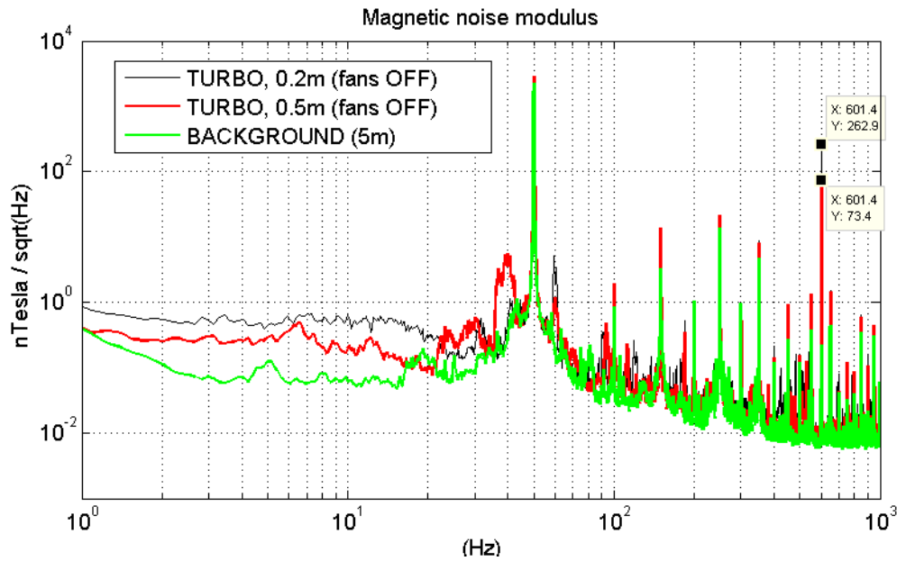
Figure 15. Turbo pump 1600 TMU: measured at 0.2m and 0.5m. Cooling fans off.
