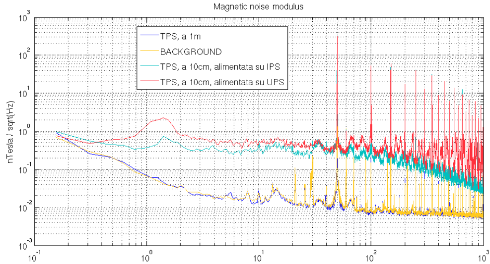
Figura 8. TPS, magnetic field noise at 1m distance (blue) and at much closer distance (light-blue and red). The red one corresponds to TPS powered on UPS.
