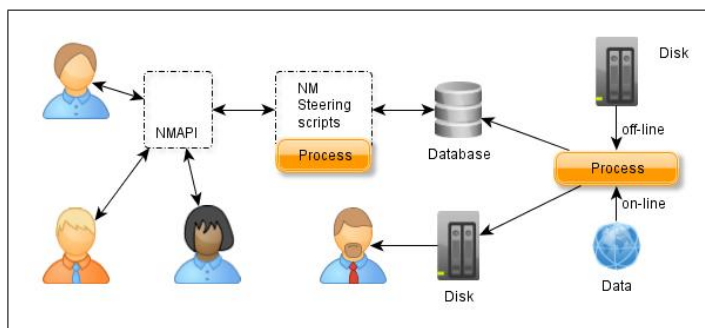
Figure 1.2: NMAPI framework
